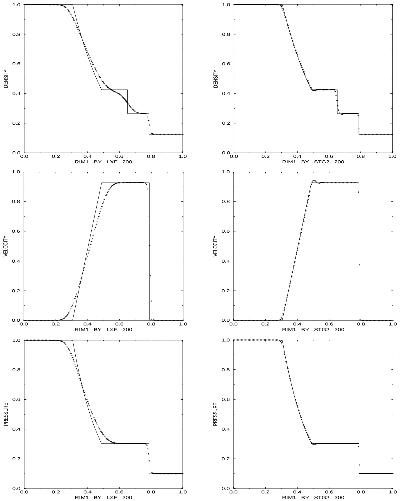
Figure 5.2: RIM1 - LXF vs. STG2
