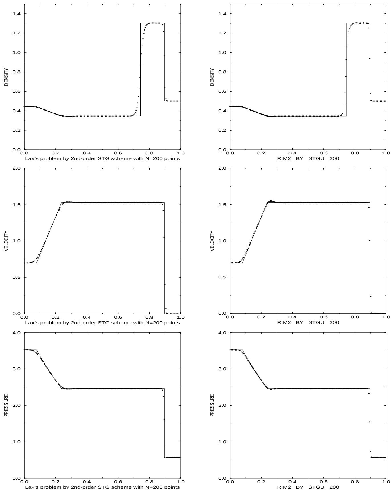
Figure 5.7: RIM2 - STG vs. STGU
