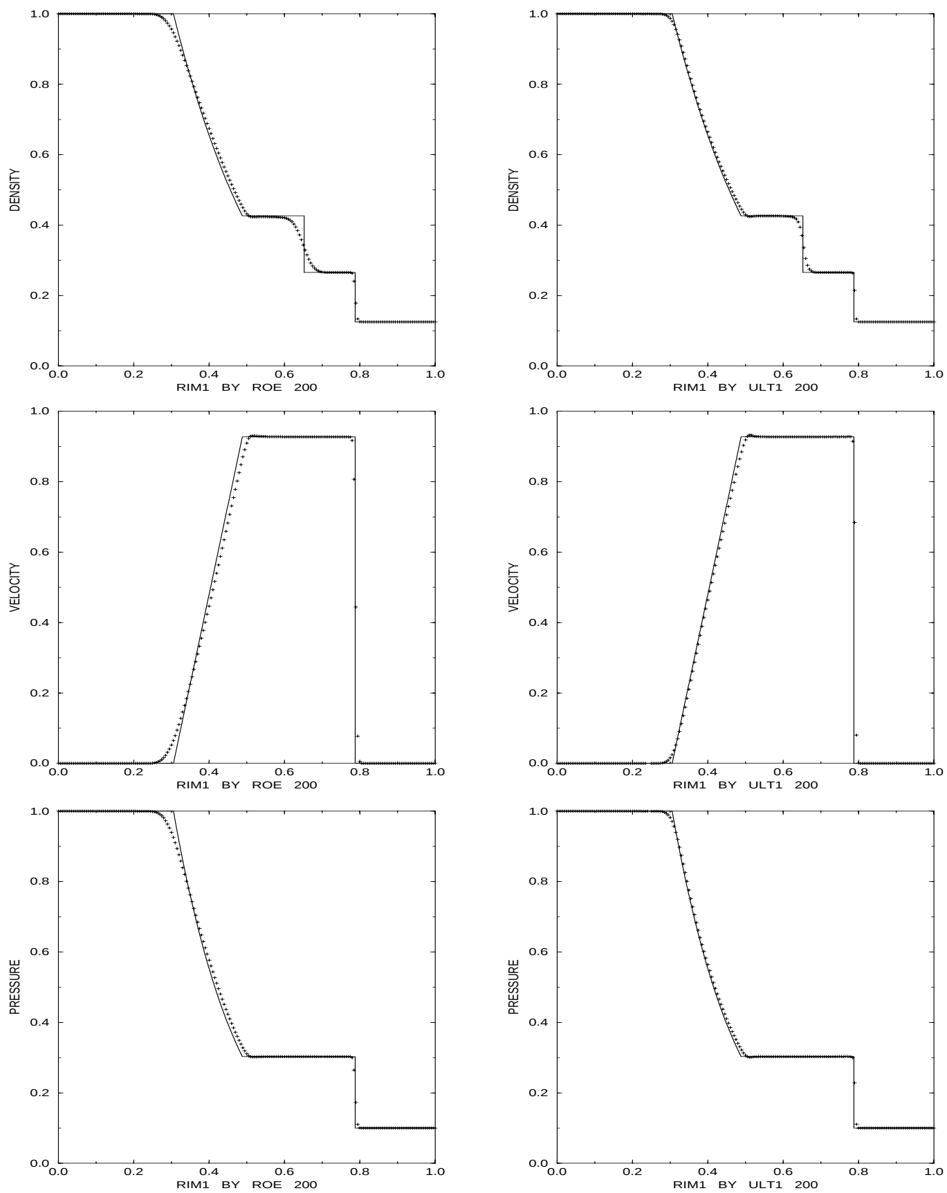
Figure 5.1: RIM1 - ROE vs. ULT1
