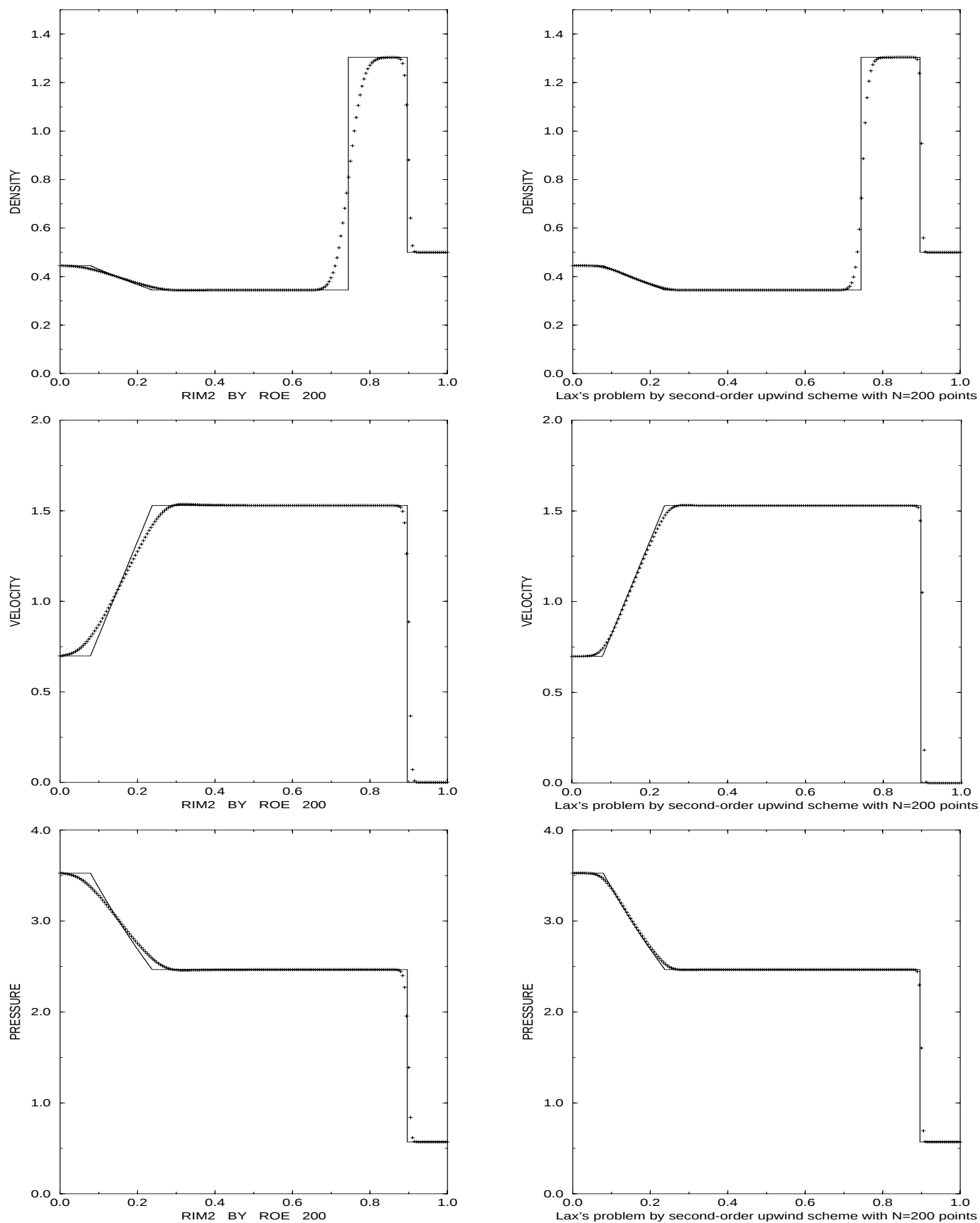
Figure 5.5: RIM2 - ROE vs. ULT1
