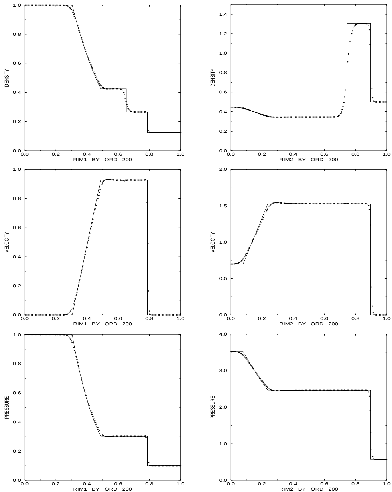
Figure 5.9: RIM1 and RIM2 by ORD
