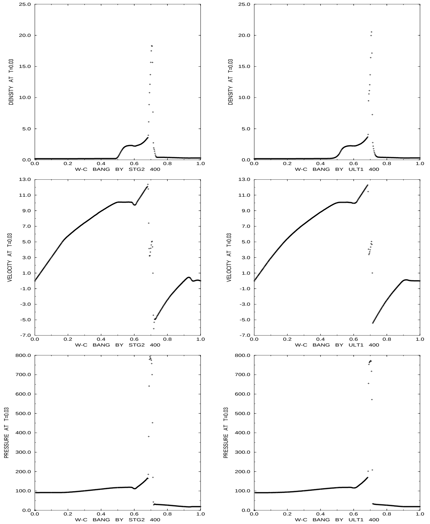
Figure 5.14: WC-BANG T=0.03 - STG2 vs. ULT1
