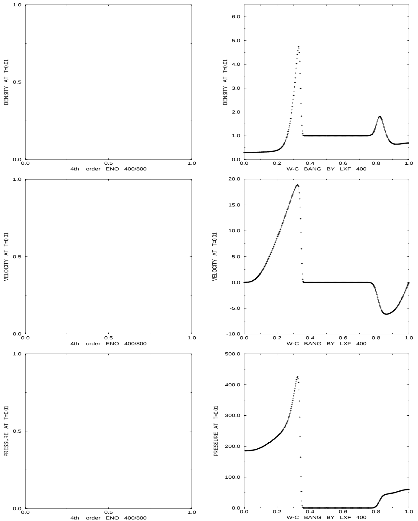
Figure 5.10: WC-BANG T=0.01 - ENO vs. LXF (the ENO results are in [9])
