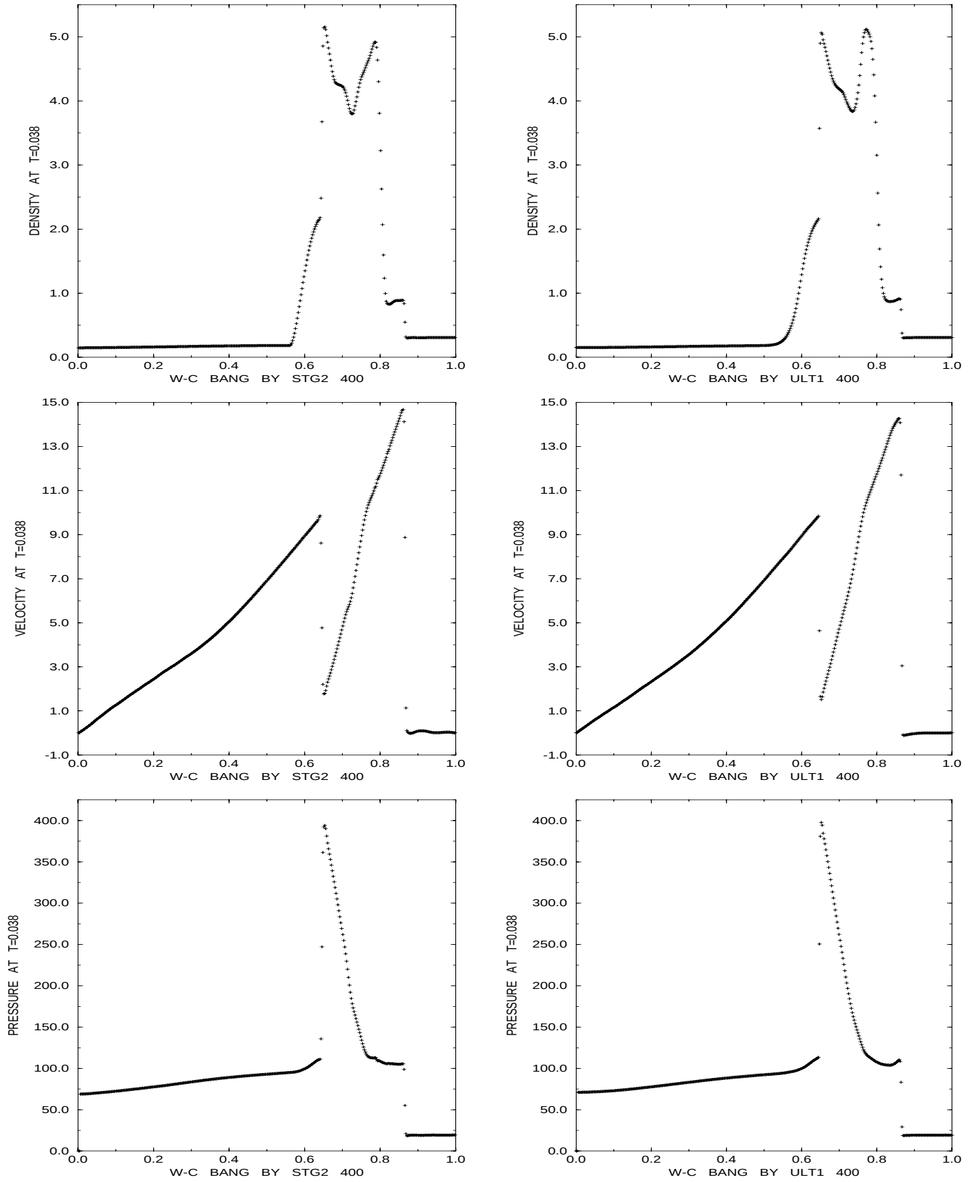
Figure 5.15: WC-BANG T=0.038 - STG2 vs. ULT1
