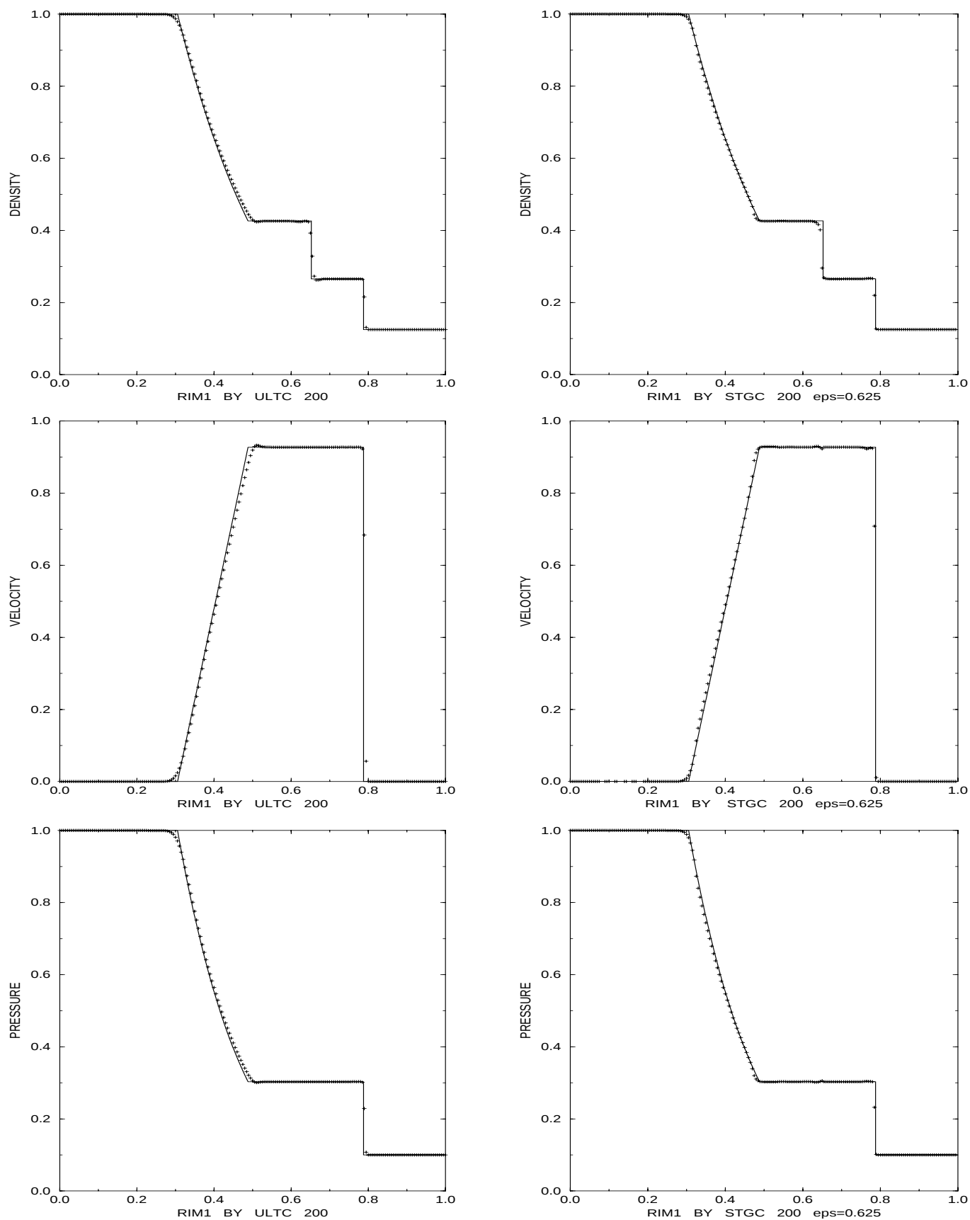
Figure 5.4: RIM1 - ULTC vs. STGC
