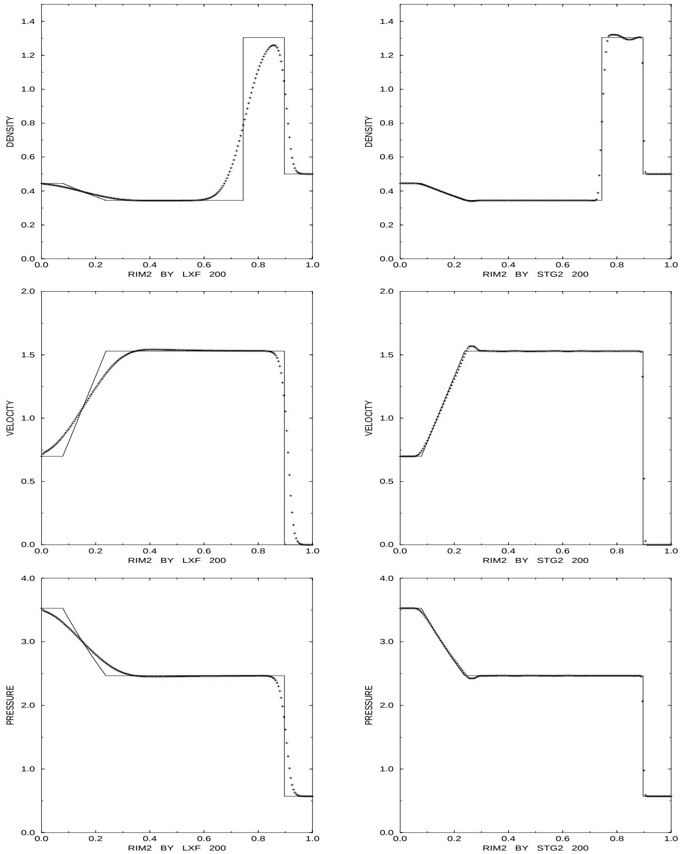
Figure 5.6: RIM2 - LXF vs. STG2
