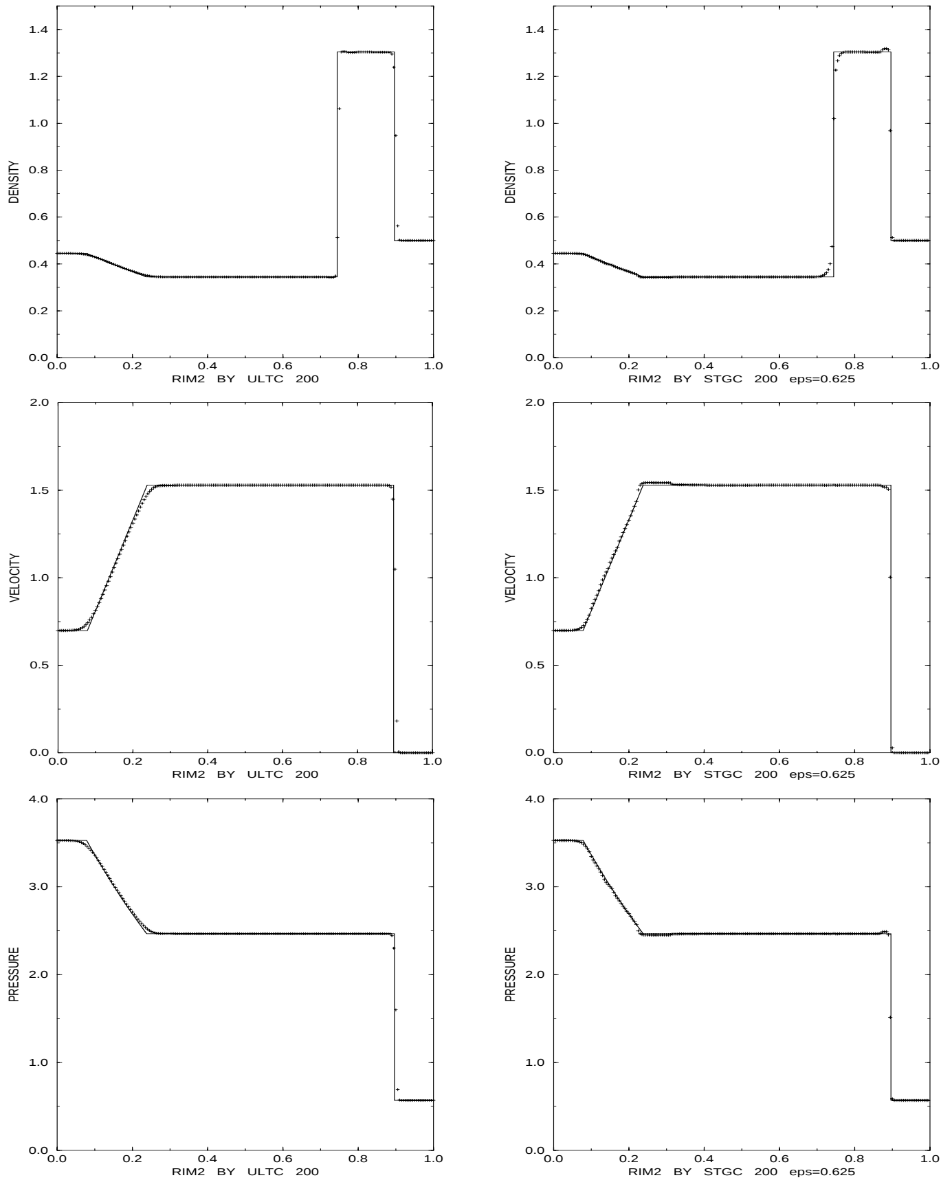
Figure 5.8: RIM2 - ULTC vs. STGC
