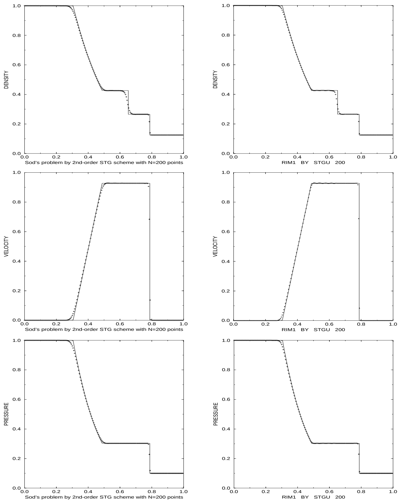
Figure 5.3: RIM1 - STG vs. STGU
