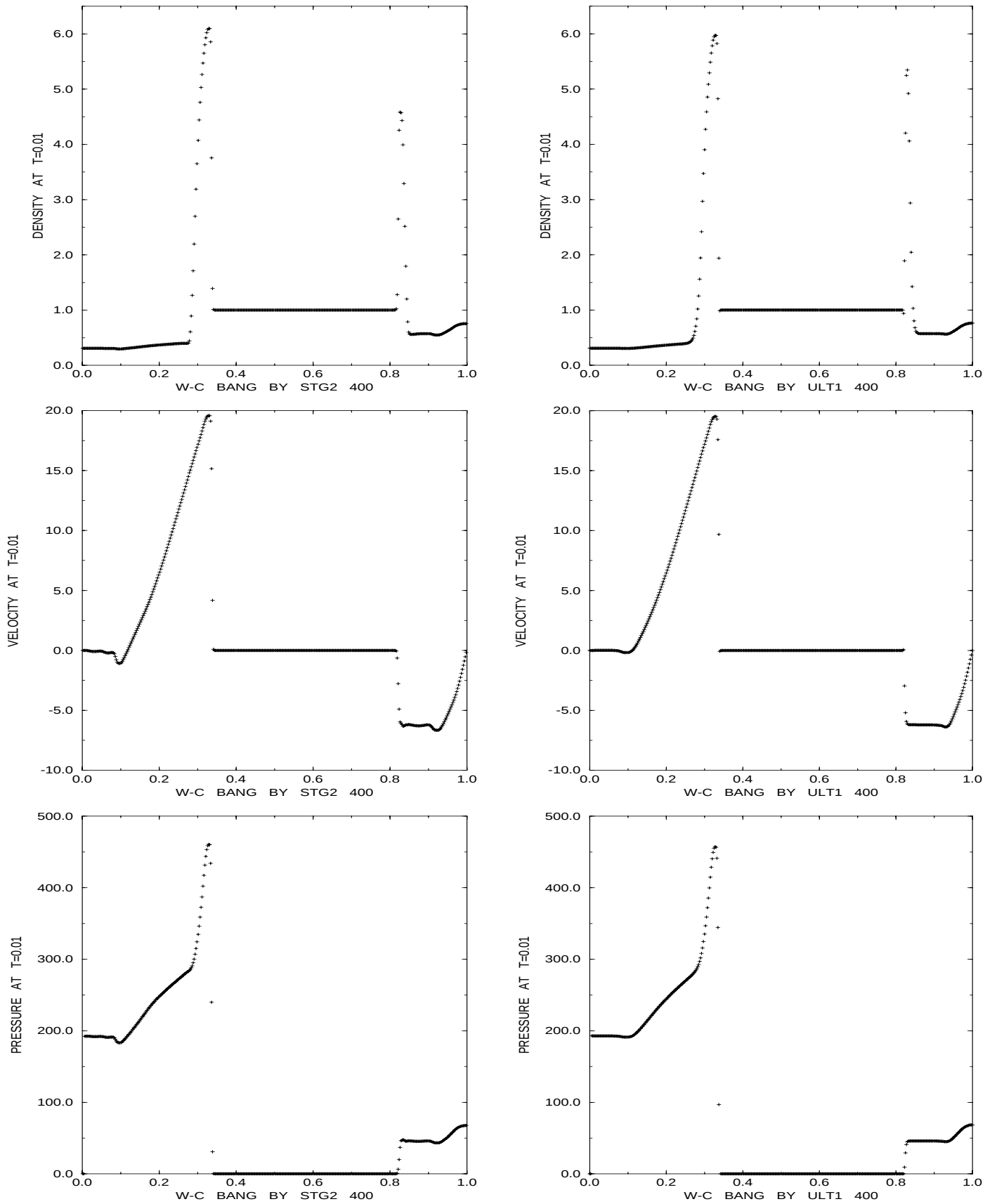
Figure 5.13: WC-BANG T=0.01 - STG2 vs. ULT1
