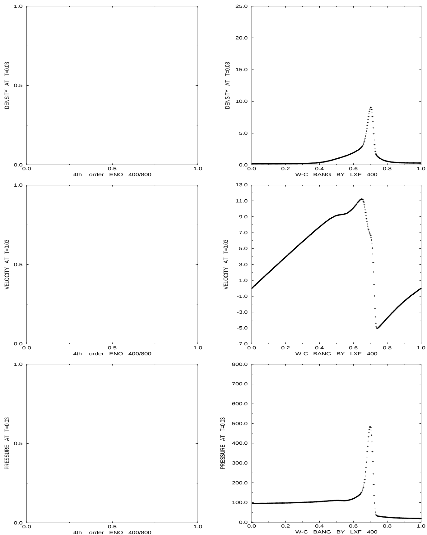
Figure 5.11: WC-BANG T=0.03 - ENO vs. LXF (the ENO results are in [9])
